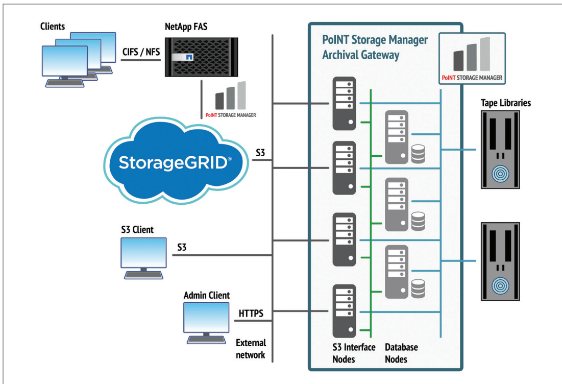
DIAGRAM 1: POINT STORAGE MANAGER ARCHIVAL GATEWAY ENABLES ADVANCED ARCHIVING ON TAPE FOR NETAPP STORAGEGRID WEBSCALE.
